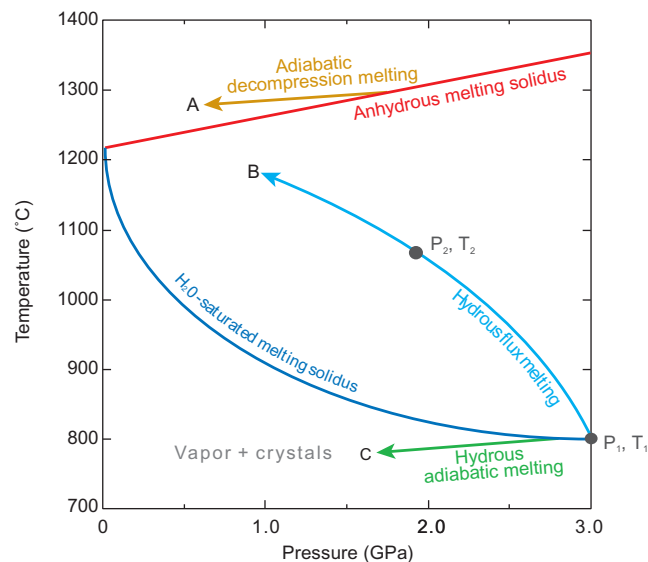
Figure 9 Schematic diagram showing the anhydrous and H 2 O-saturated solidi for mantle peridotite (curves) and illustrating several possible paths for melting generation in the mantle wedge (arrows) (Gaetani and Grove, 2003). A, adiabatic decompression melting; B, hydrous flux melting; C, hydrous adiabatic melting.
