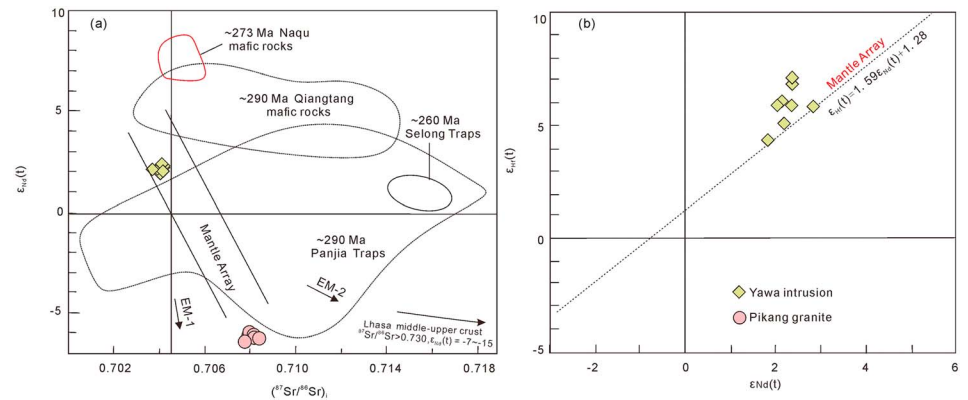
Figure 8. (a) Whole-rock ^{87}\text{Sr}/^{86}\text{Sr} versus \epsilon_{\text{Nd}}(t) and (b) \epsilon_{\text{Nd}}(t) versus \epsilon_{\text{Hf}}(t) diagrams for the Yawa intrusions. Data sources are as follows: Pikang granite from Zhu et al. (2009), Lhasa middle-upper continental crust is the Ningzhong strongly peraluminous granites and Amdo orthogneiss (Liu et al., 2006; Xu et al., 1985), \sim 273 -Ma Naqu mafic rocks are from Chen et al. (2017), Qiangtang mafic rocks from Zhang and Zhang (2017), \sim 260 Ma Selong Traps from Zhu et al. (2010), Panjal traps from Shellnutt, 2018), and mantle array from Chauvel and Blichert-Toft (2001).
