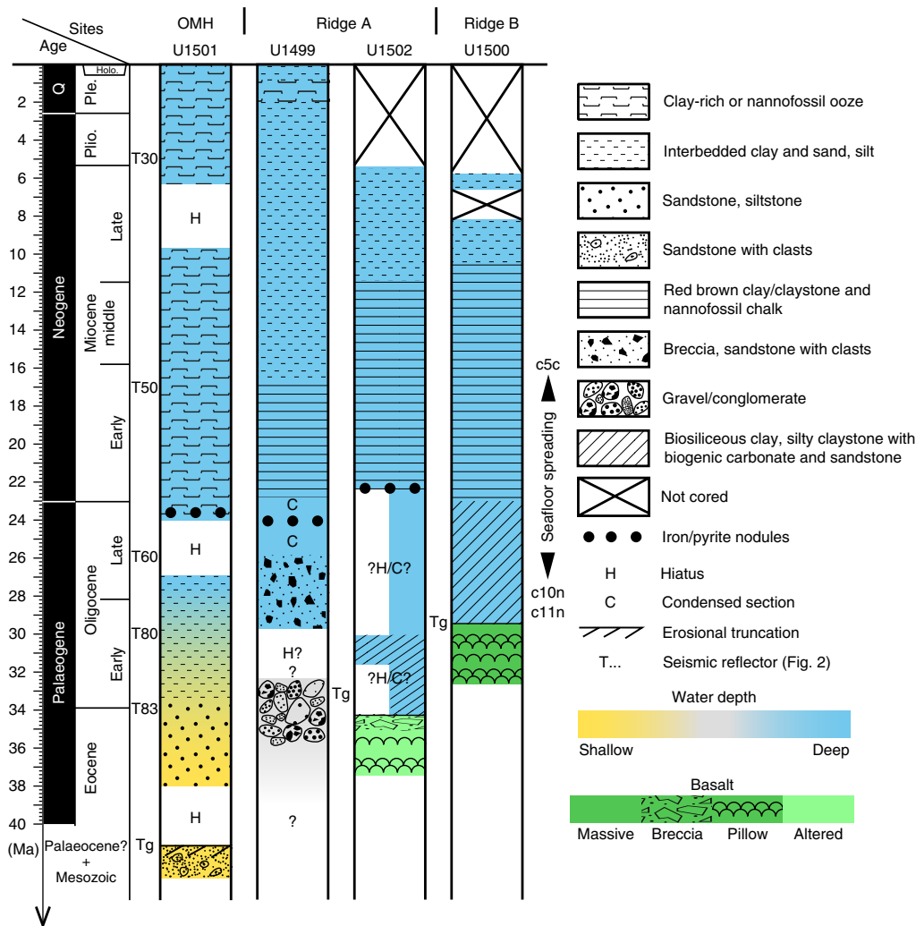
Fig. 3 | Summary chart of drilling results. Ages based on core samples analysed for calcareous nanfossils, foraminifers, diatoms and ostracods. Lithostratigraphy is from detailed core descriptions 29,32–34 following the GTS12 48 geological timescale.
