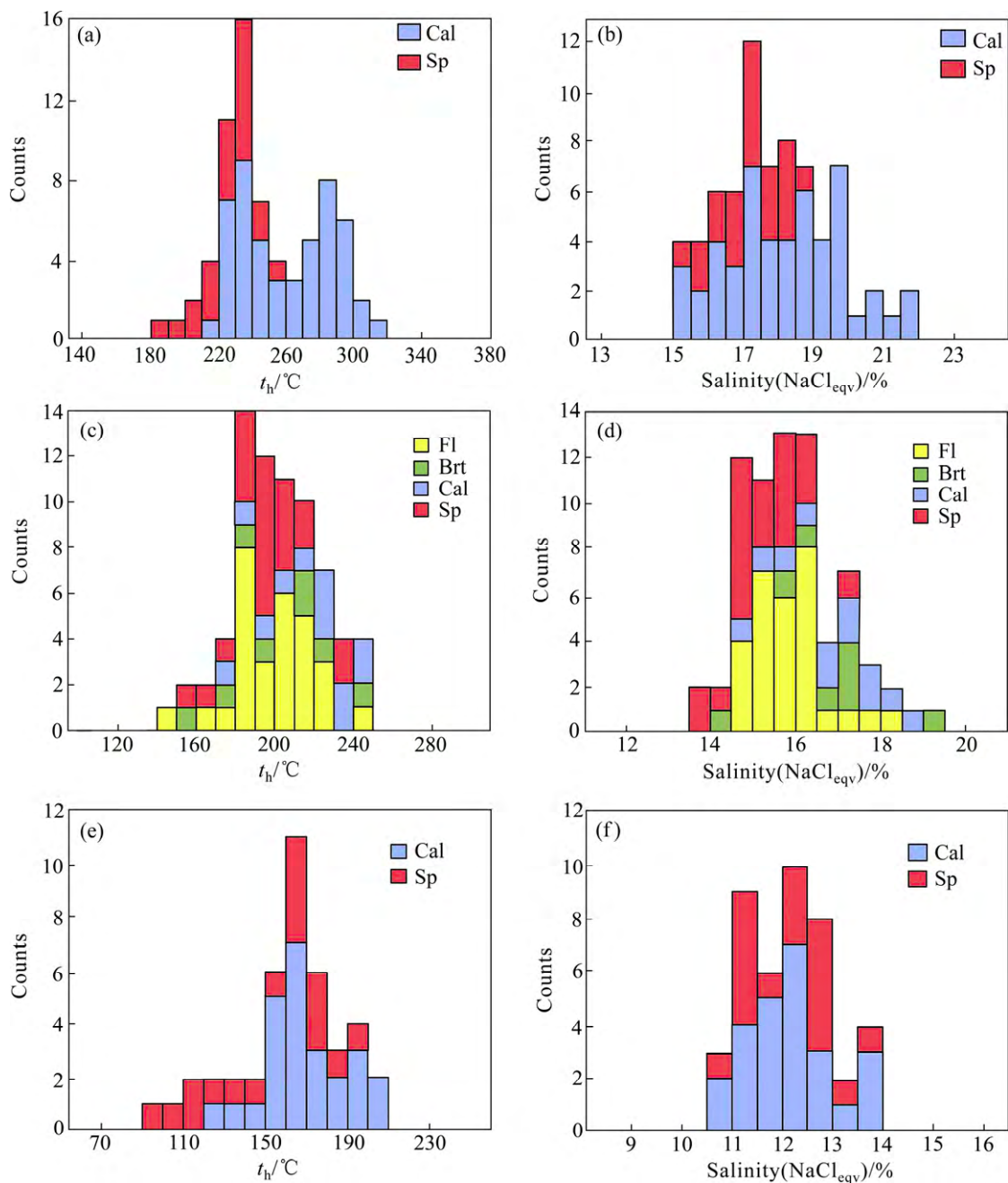
图 7 土地坪铅锌矿床 Ia 型流体包裹体均一温度、盐度分布直方图: Cal—方解石; Brt—重晶石; Fl—萤石; Sp—闪锌矿 Fig. 7 Histogram of homogenization temperature and salinity of type Ia fluid inclusions from Tudiping Pb-Zn deposit: Cal—Calcite; Brt—Barite; Fl—Flourite; Sp—Sphalerite
