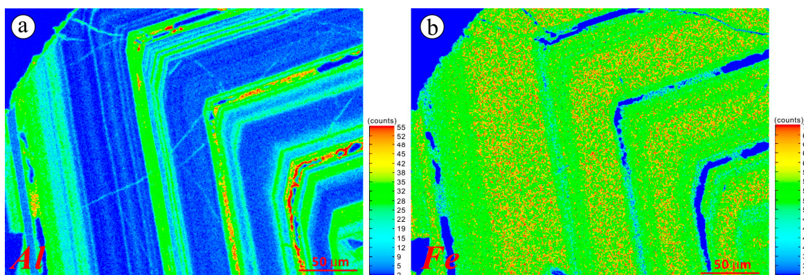
Figure 7. EPMA element mapping of (a) Fe and (b) Al for a dark red garnet particle.
