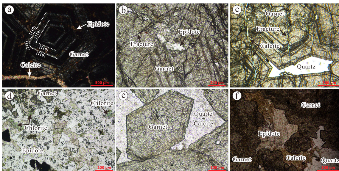
Figure 5. Photomicrographs showing representative textural features of the garnets from the Yongping deposit. (a) Dark red garnet particle locally shows a morphological transition from simple dodecahedral {110} growth in the core to composite dodecahedral {110}–trapezohedral {211} growth near its margin in the rim, and it is cut by a calcite vein (CPL); (b) dark red garnet particle is locally cut by later fractures and corroded by epidote (PPL); (c) green garnet particle has obvious oscillatory zones and is cut by a calcite vein, and the quartz occurring between the garnet particles (PPL) shows an anhedral granular texture; (d) green garnet particle with an anhedral granular texture resulted from corrosion by quartz, and the epidote has an anhedral granular texture and is replaced by chlorite (PPL); (e) light brown garnet particle with an euhedral granular texture, and calcite and quartz between the garnet particles (PPL); and (f) light brown garnet particle with a subhedral granular texture. Epidote, calcite and quartz usually occur between garnet particles, and epidote locally is replaced by calcite (PPL).
