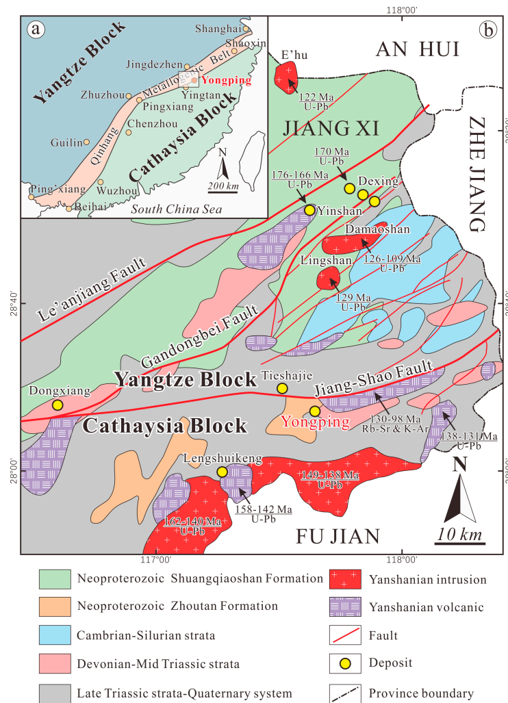
Figure 1. Regional geology of the northeastern Jiangxi district and the location of the Yongping Cu deposit (modified after [27]).
