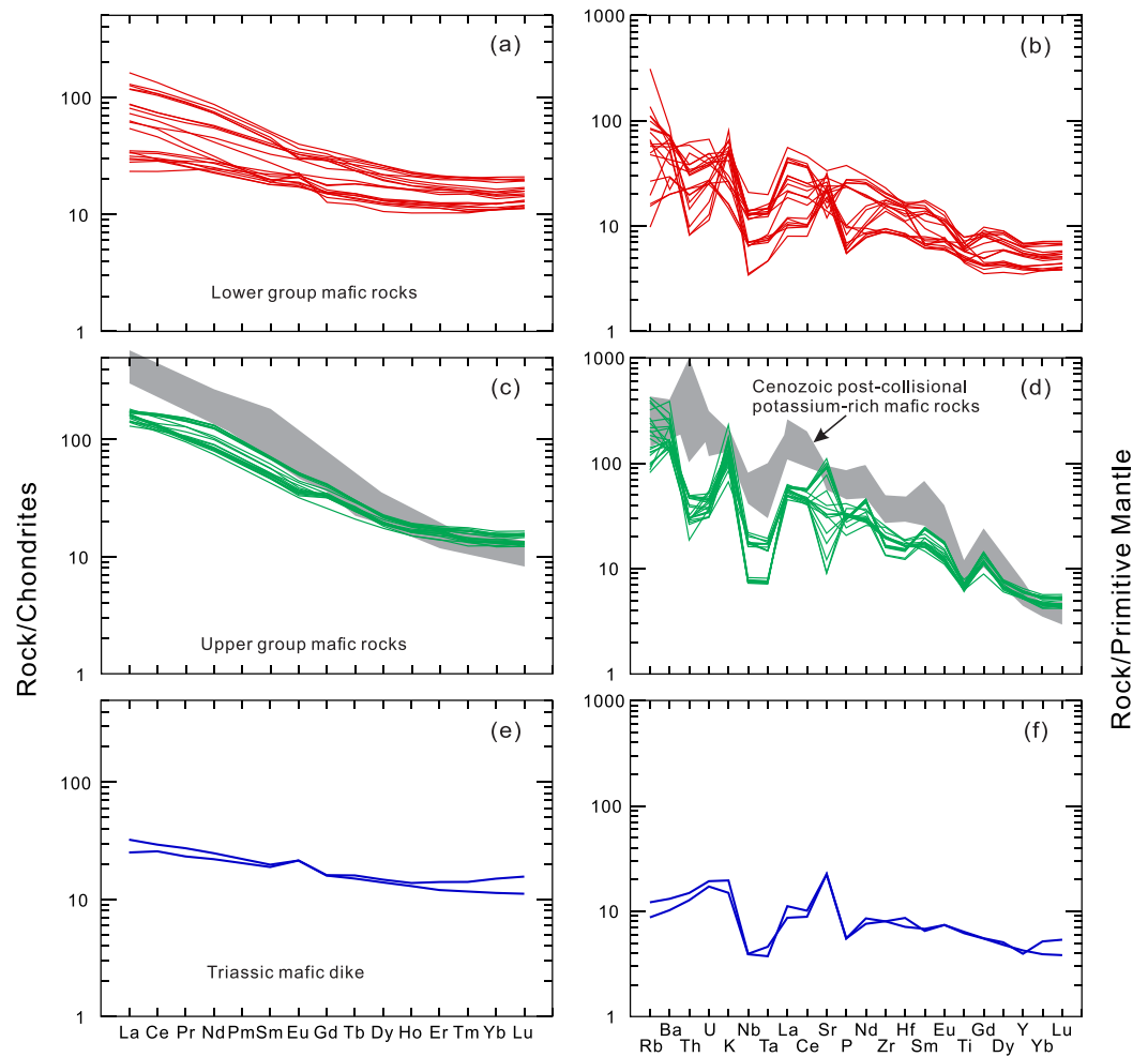
Figure 5. Chondrite-normalized rare earth element patterns and primitive mantle-normalized multi-element diagram for the early Permian-Triassic magmatic rocks of the Awulale Mountains. Chondrite and primitive mantle normalizing values are from Sun and McDonough (1989). Cenozoic post-collisional potassium-rich mafic rocks (Guo et al., 2014) are shown for comparison. The data sources are same as Figure 4.
