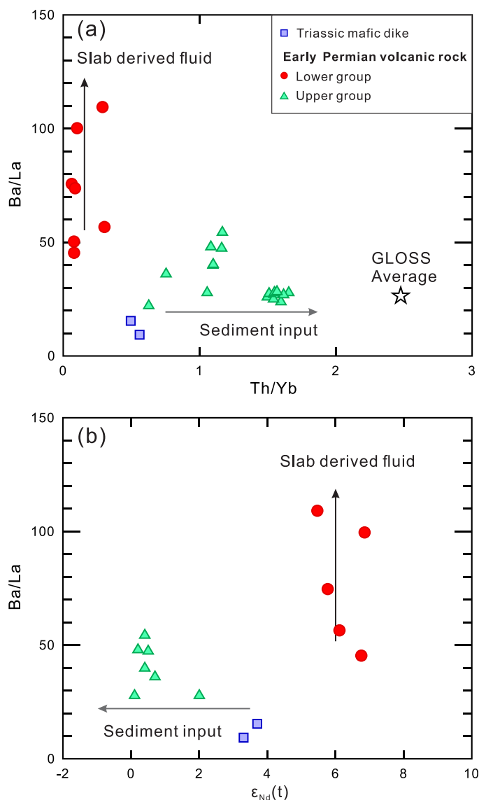
Figure 7. (a) Ba/La versus Th/Yb and (b) Ba/La versus \epsilon_{Nd}(t) plots. GLOSS average are from Plank and Langmuir (1998). The data sources and symbols are same as Figure 4.
