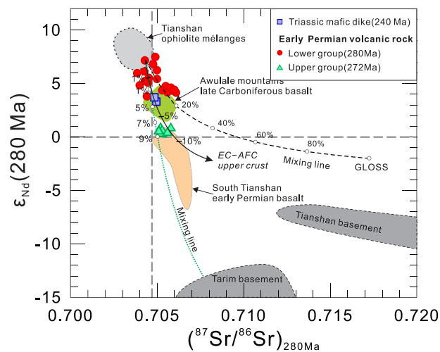
Figure 6. (^{87}\text{Sr}/^{86}\text{Sr})_i versus \epsilon_{\text{Nd}}(t) diagram showing two-component mixing and EC-AFC calculations. The Sr-Nd isotope data of Tianshan ophiolites (Xu et al., 2006); late Carboniferous basalts from the Awulale Mountains (Li et al., 2015; Tang et al., 2014; Yan et al., 2015) and South Tianshan early Permian basalts (Huang et al., 2015; Liu et al., 2014) are shown for comparison. Tarim Archean and Neoproterozoic basement are from Cao et al. (2011). Tianshan Neoproterozoic basement are from Chen et al. (1999). Data for global subducting sediment (GLOSS) are from Plank and Langmuir (1988). The modeling parameters are listed in supporting information Table S3. Small circles on the curves indicate the percentage of assimilated contaminant. The other data sources and symbols are same as Figure 4.
