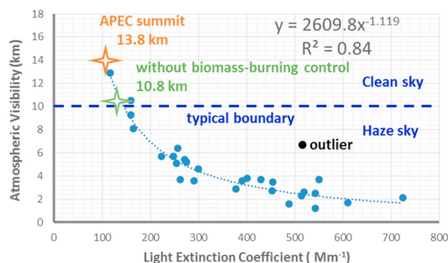
Figure 5. Atmospheric visibility during APEC summit with and without biomass-burning control. The established correlation between atmospheric visibility and light extinction coefficient was based on the data set in Tao et al. [2009]. One outlier datum was excluded.
