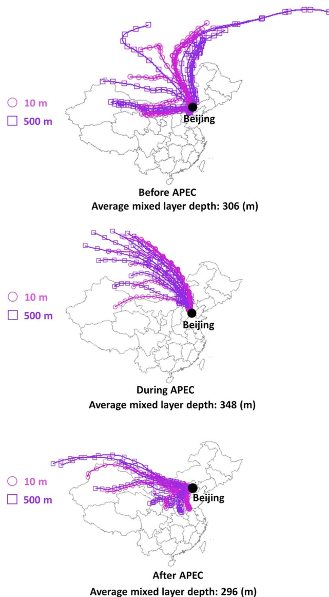
Figure 3. The 72 h back trajectories at 10 m and 500 m aboveground level and average mixed layer depth (top) before, (middle) during, and (bottom) after the APEC summit. All these data were obtained from Air Resources Laboratory, NASA.
