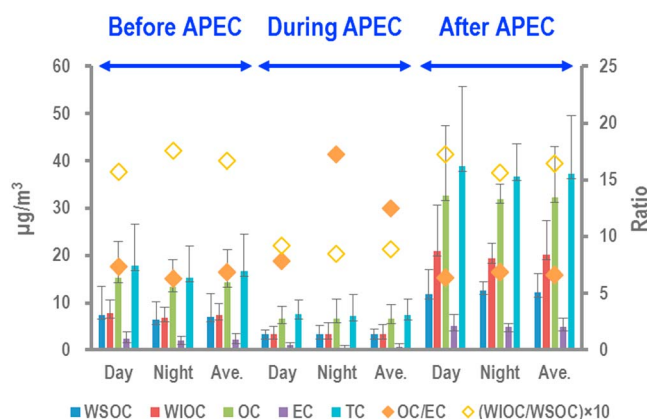
Figure 2. Concentrations of carbon fractions (left Y axis) and the ratios of OC/EC and WIOC/WSOC (right Y axis) during the sampling campaign.
