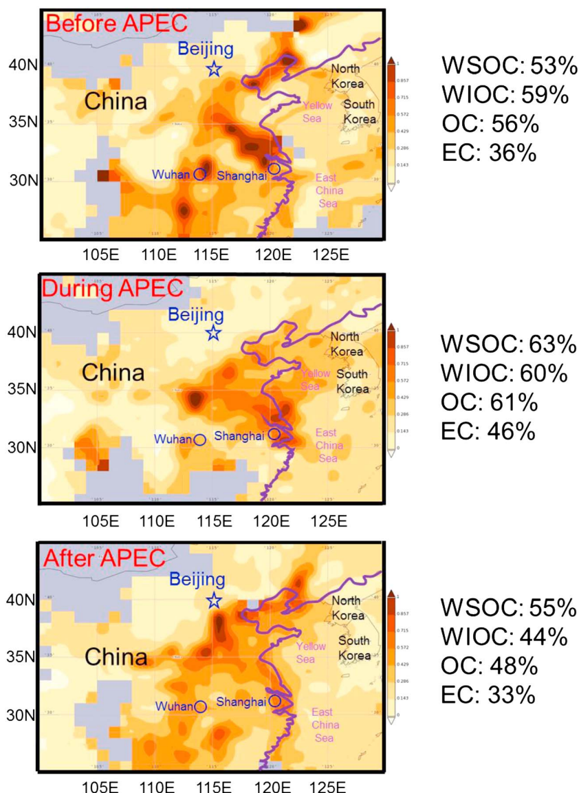
Figure 1. Map showing the geographic location of Beijing in China and the average aerosol optical depth (AOD) and the contribution of nonfossil sources to different carbon fractions (top) before, (middle) during, and (bottom) after APEC summit.
