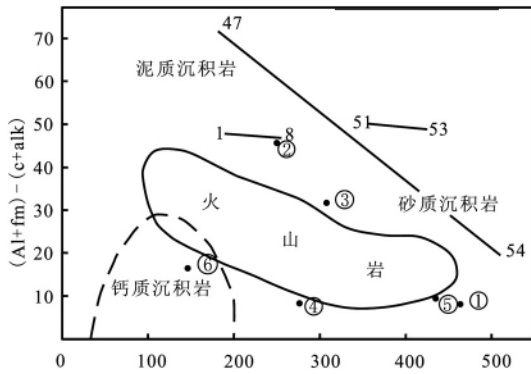
图5 (al+fm)-(c+alk)-Si 图解
