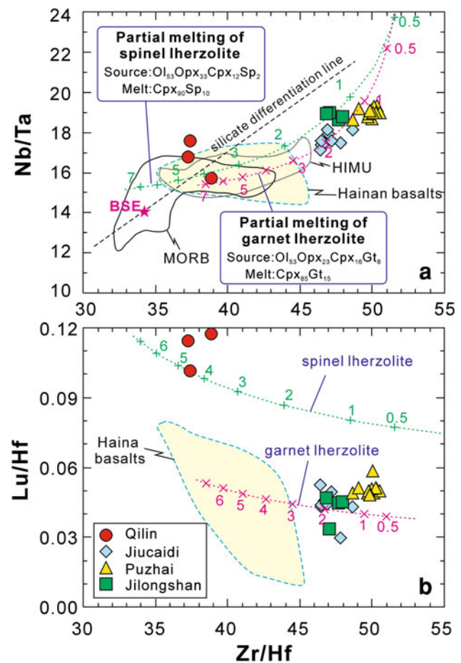
Fig. 6 Nb/Ta and Lu/Hf vs. Zr/Hf of the eastern Guangdong Cenozoic basalts. The silicate differentiation line indicates a first-order coupling of Nb/Ta and Zr/Hf fractionation in terrestrial reservoirs (Münker et al. 2003). The assumed source of non-modal batch melting curves is “99 % primitive mantle + 1 % crust”, except for Hf, for which the concentration in the primitive mantle was elevated from 0.3 to 0.38 ppm to fit the requirement of a lower Zr/Hf ratio (Pfänder et al. 2007). Both the primitive mantle and crust values are from Palme and O’Neill (2003). The numbers of the curves denote degree of melting in percent, using the partition coefficients of McDade et al. (2003) (Ol, Opx, Cpx), Westrenen et al. (1999) (Gt) and Elkins et al. (2008) (Sp). HIMU and MORB from Pfänder et al. (2007), BSE value from Münker et al. (2003)
