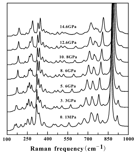
Fig. 2 Representative Raman spectra of PbWO 4 -III under ambient and high pressures at room temperature
