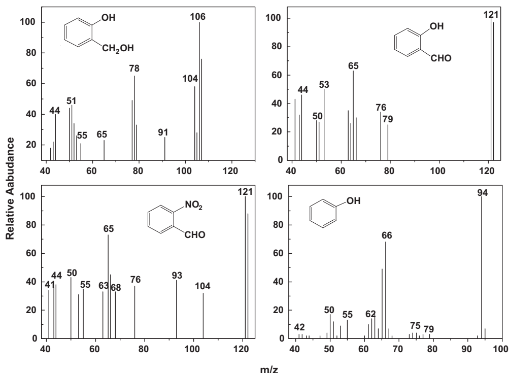
Fig. 6. Mass spectra of adsorbed intermediates on TiO 2 thin film during the photocatalytic degradation identified by GC-MS without silylation.
