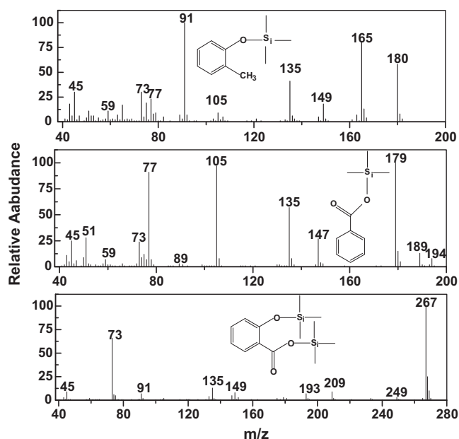
Fig. 7. Mass spectra of adsorbed intermediates on TiO 2 thin film during the photocatalytic degradation identified with BSTFA silylation.
