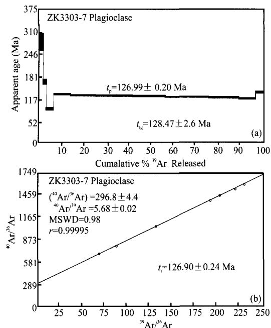
Fig. 7. The ^{40}\text{Ar}/^{39}\text{Ar} spectra (a) and corresponding isochron diagrams of plagioclase in Shaxi porphyrite intrusive, the south Tan-Lu fault belt (Sample 3303-07).
