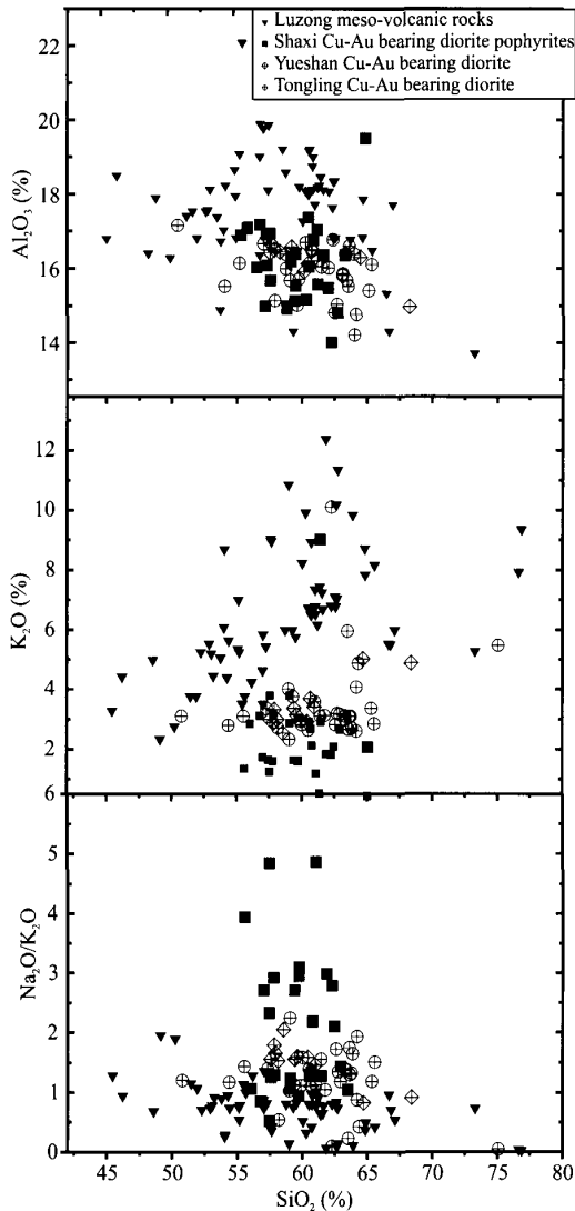
Fig. 3. \text{SiO}_2 vs. \text{Al}_2\text{O}_3 , \text{K}_2\text{O} and \text{Na}_2\text{O}/\text{K}_2\text{O} diagrams showing variations of different igneous rock associations related to Cu-Au mineralization in Anhui Province (after Rollinson, 1993 and Rickwood, 1989; data are derived from the No. 327 Geological Party, 1982; the No. 321 Geological Party, 1990; Bureau of Geology and Mineral Resources of Anhui Province, 1987; Chang et al., 1991; Ren et al., 1991; Qiu, 1992; Yang, 1996; Wang and Yang, 1996; Yang et al., 2001b).
