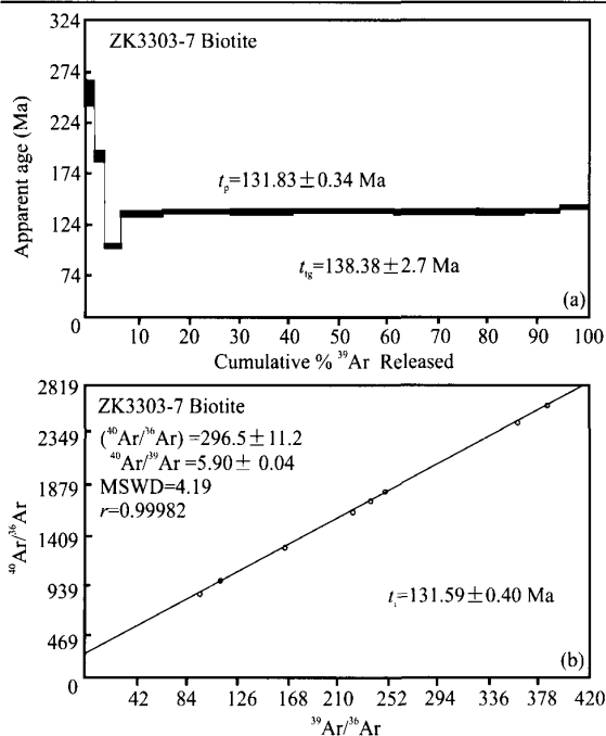
Fig. 6. The ^{40}\text{Ar}/^{39}\text{Ar} spectra and corresponding isochron diagrams of biotite in the Shaxi porphyrite intrusive, the southern Tan-Lu fault belt (Sample 3303-07).
