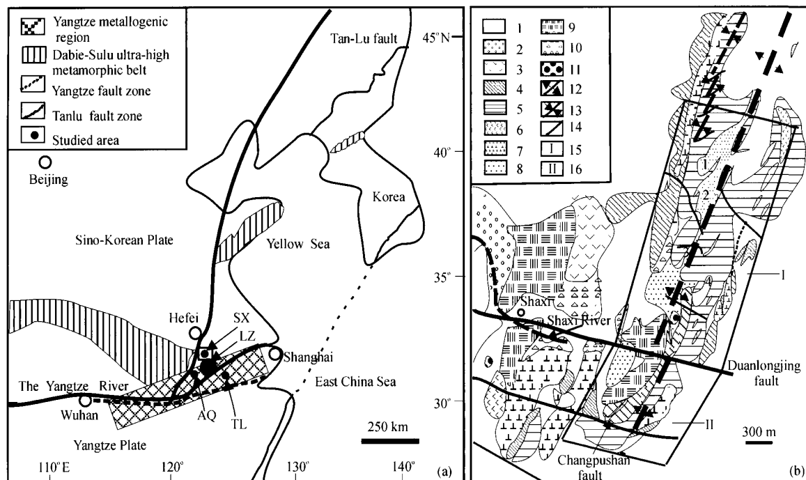
Fig. 1. The regional geological and tectonic map of the studied area.
