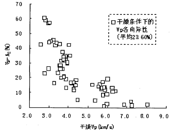
图 4 干燥条件岩石纵波各向异性随 VP 变化关系 Fig. 4 Variation of VP-anisotropy with compressional wave velocity at dry condition
