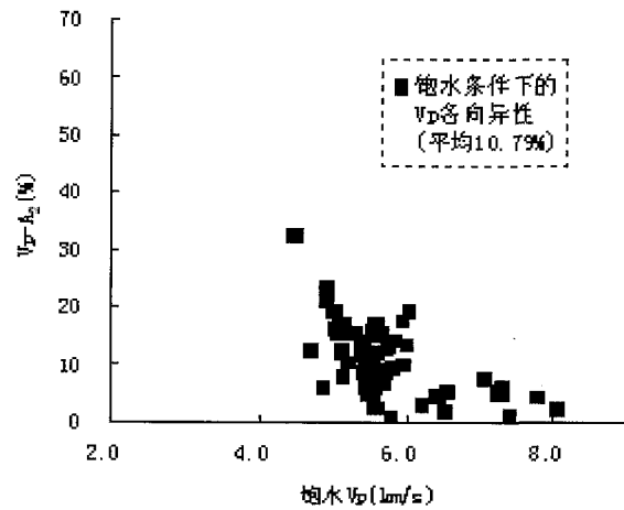
图 5 饱水条件纵波各向异性随 V_p 的变化关系 Fig. 5 Variation of V_p -anisotropy with compressional wave velocity at water-saturated condition
