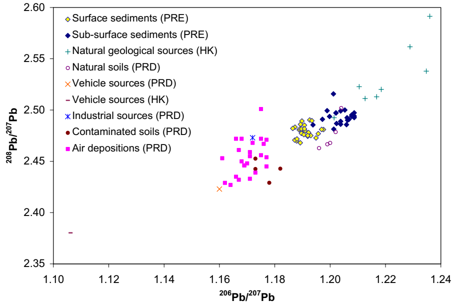
Fig. 7. The correlation between ^{208}\text{Pb}/^{207}\text{Pb} and ^{206}\text{Pb}/^{207}\text{Pb} of sediments in the PRE (this study), atmospheric deposition (Wong et al., 2003) and soils (Wong, 2002) in the PRD as well as natural geological sources and anthropogenic sources in the PRD (Zhu et al., 2001) and Hong Kong (Duzgoren-Aydin et al., 2004; this study).
