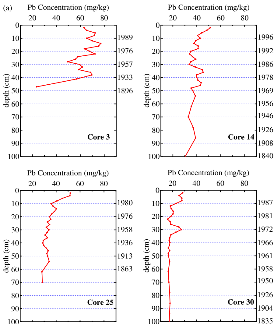
Fig. 4. The profile of (a) Pb, (b) Zn, (c) Cu, (d) Ni and (e) Fe concentrations over time in Cores 3, 14, 25, and 30.
