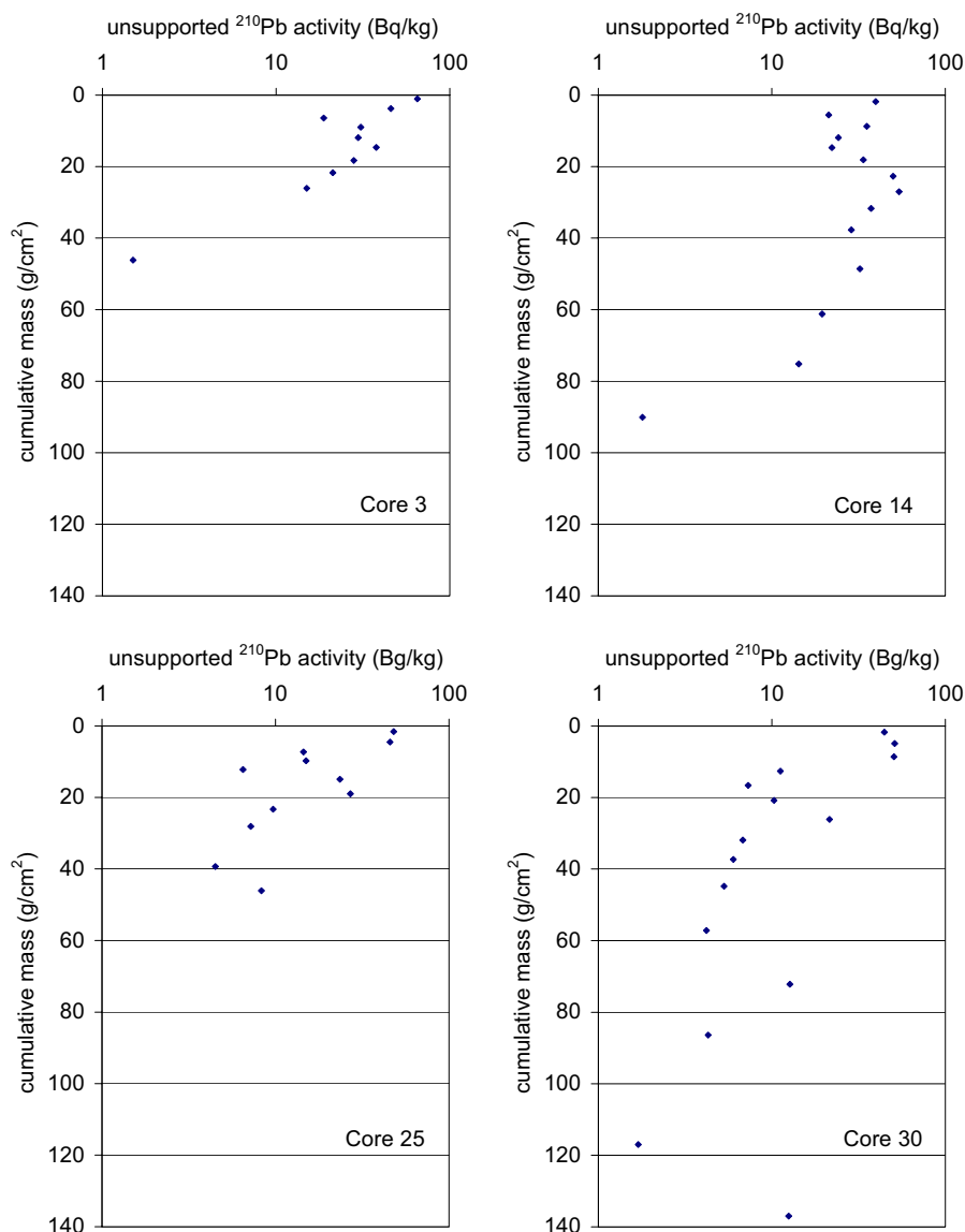
Fig. 2. The unsupported 210 Pb activities in Cores 3, 14, 25 and 30.
