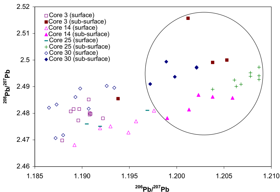
Fig. 5. The correlation between ^{208}\text{Pb}/^{207}\text{Pb} and ^{206}\text{Pb}/^{207}\text{Pb} of surface and sub-surface sediments in the PRE.
