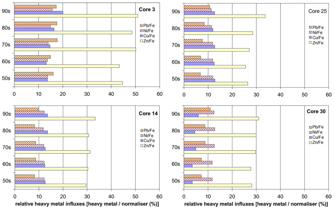
Fig. 8. The relative influxes of Pb, Ni, Cu and Zn normalised by Fe in every decade in (a) Core 3, (b) Core 14, (c) Core 25, and (d) Core 30 of the PRE.
