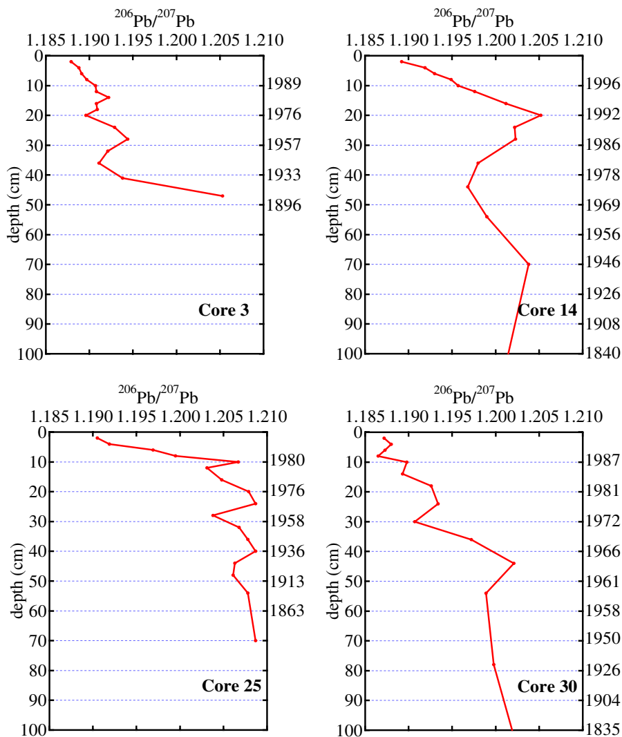
Fig. 6. The profile of ^{206}\text{Pb}/^{207}\text{Pb} over time in Cores 3, 14, 25, and 30.
