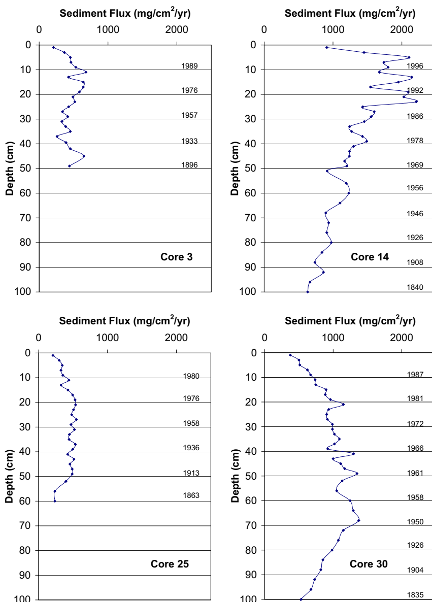
Fig. 3. The sediment flux of Cores 3, 14, 25, and 30 using the CRS model.
