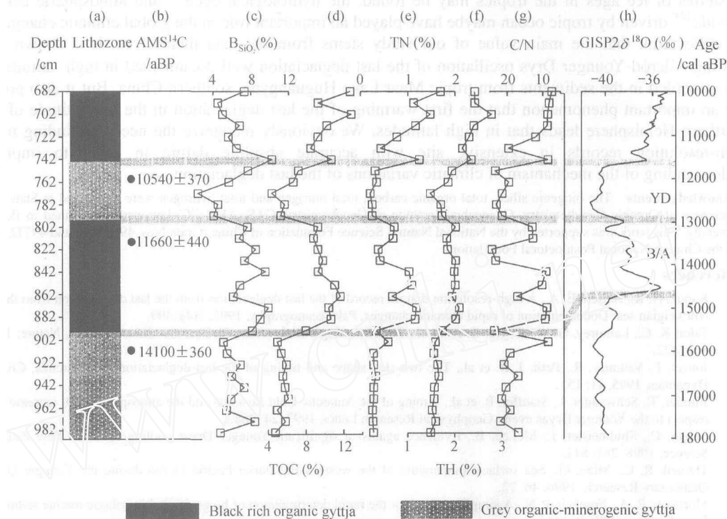
Fig. 1. The data set of core B from Maar Lake Huguangyan during the last deglaciation and comparison with GISP2 \delta^{18}\text{O} record. (a) Sediment profile; (b) AMS ^{14}\text{C} ages; (c) biogenic silica ( \text{B}_{\text{SiO}_2} ); (d) total organic carbon (TOC); (e) total nitrogen (TN); (f) total hydrogen (TH); (g) C/N; (h) GISP2 \delta^{18}\text{O} curve.
